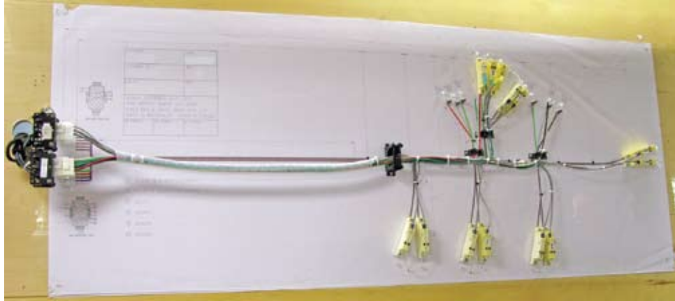
Large harnesses are tested during manufacturing on engineered assembly boards with our state-of-the-art CIRRUS testers to automatically verify continuity and isolation without fail to assure you receive a reliable, accurate, consistent product every time.
